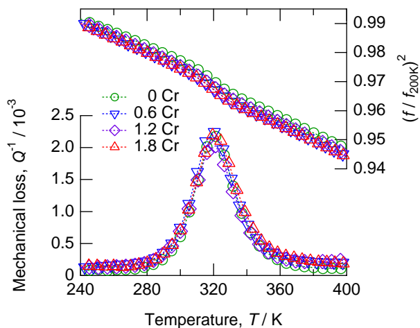
Fig. 7 The mechanical loss Q^{-1} (lower) and the square of the resonance frequency f of carburized samples containing 110 to 120 at. ppm C. The frequency is normalized to the value at 200 K.
