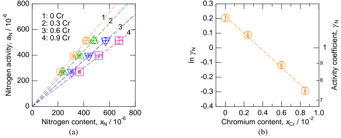
Fig. 5 (a) The same data as Fig. 4 plotted in the form of Henry's law, and (b) the activity coefficient of N as a function of Cr concentration.
