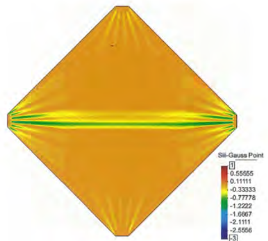
Fig. 7: Minor stress distribution by FEM analysis
